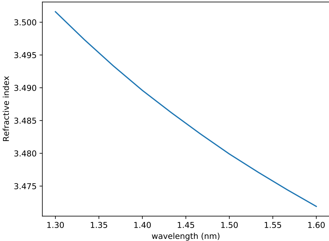
Silicon refractive index
