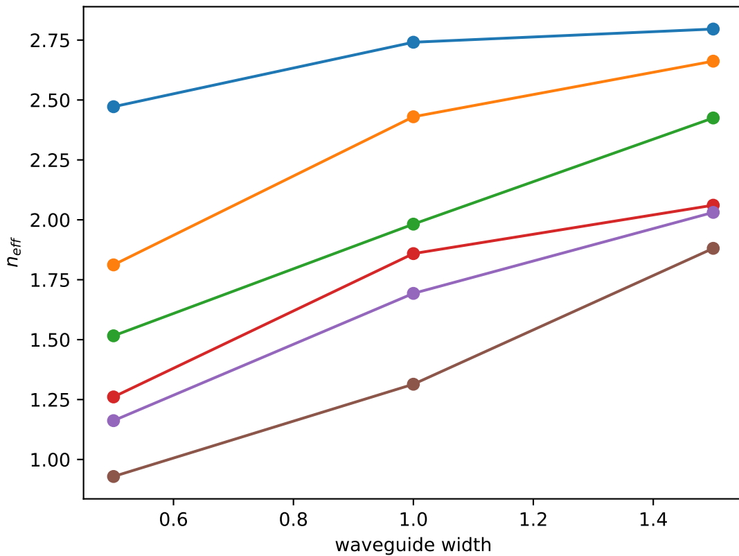
n_{eff} @ 1.55
