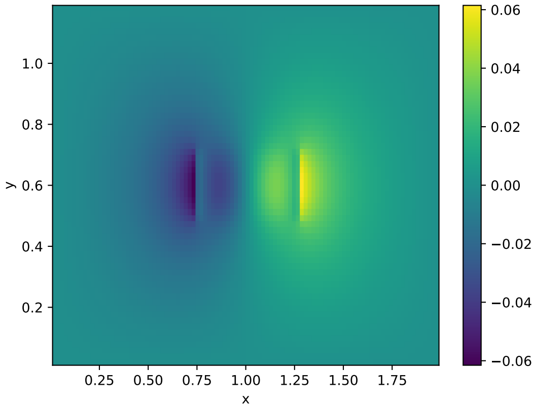
Mode 1 |E_x| Profile, n_{eff} : 1.472, \lambda = 1.550\mu\text{m}
